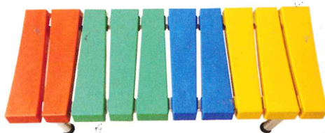
Item no. : T-26 Type: Locker Bench Materials: Base is #304 stainless, Surface is glass fiber reinforced plastics Dimension(mm): 1500(L)*450(W)*450(H) Weight: 16KGS
