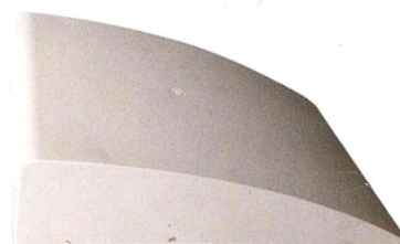
Item no. : T-25 Type: Slanting Top Material: HIPS Features: Keep dust from accumulating on top of lockers. Prevent items from being placed on top of the lockers. Dimension (cm) for T-380 Series 49.7(L)*38.3(W)*14.8(H) Dimension (cm) for T-280 Series 38(L)*28(W)*13.5(H)
